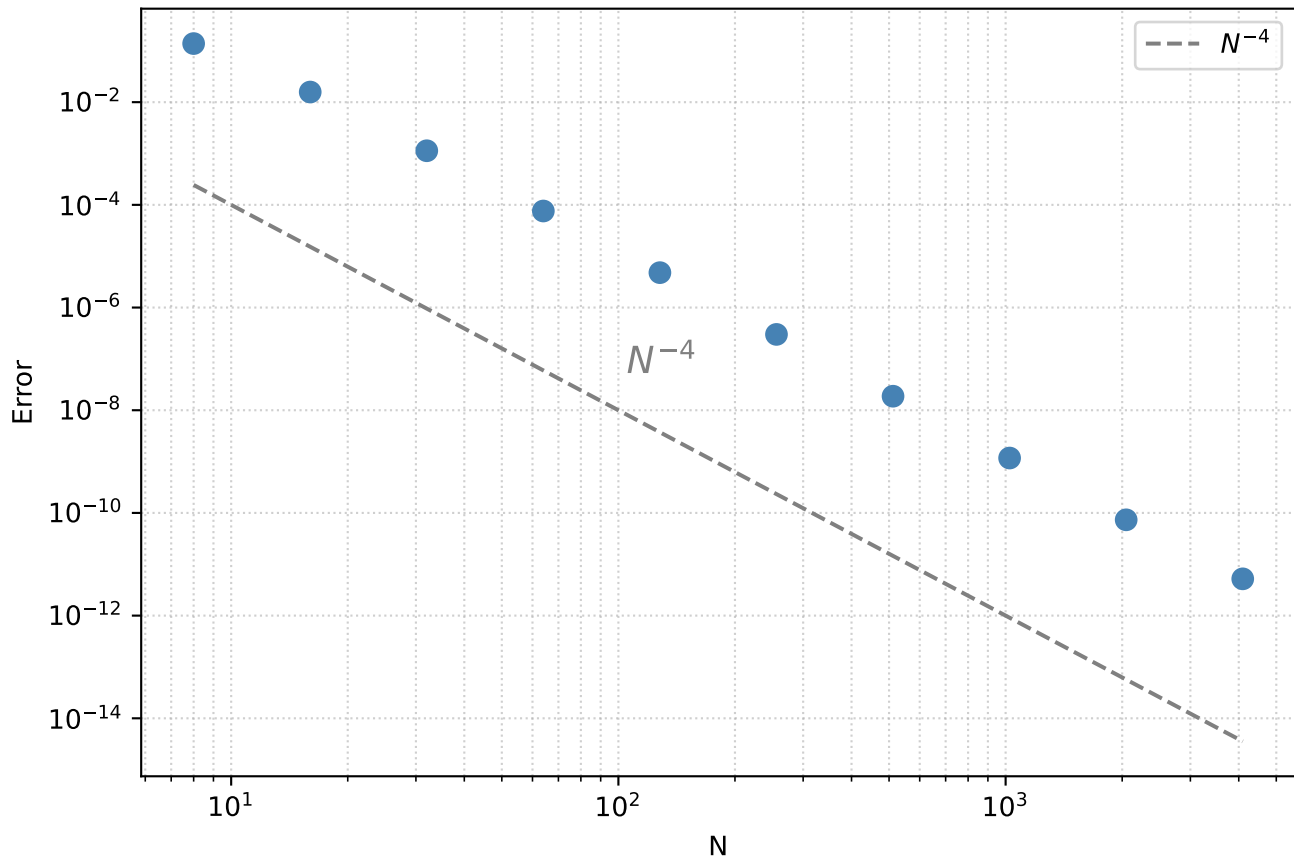
Convergence of 4th-order finite differences
